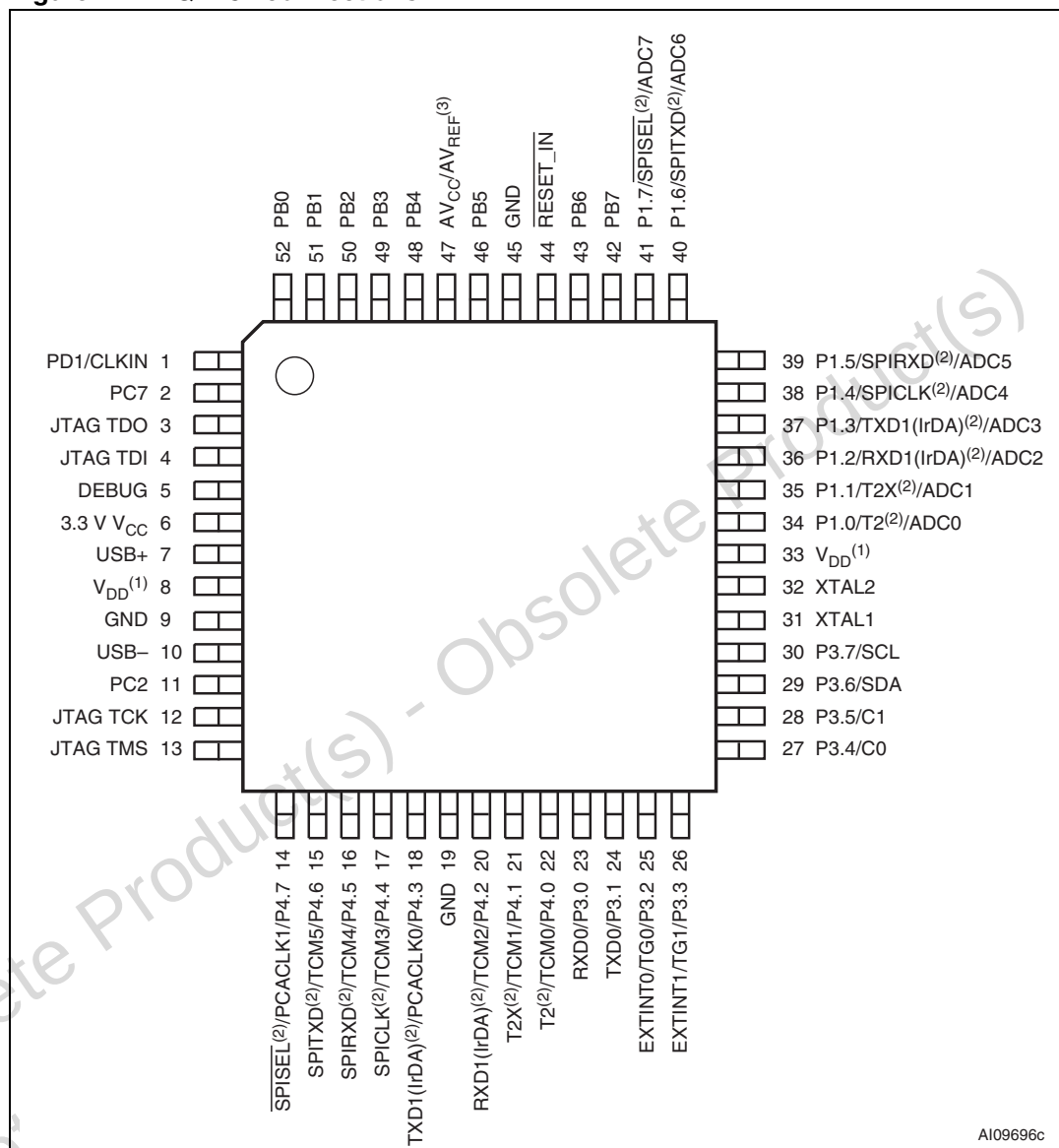
Figure 2. LQFP52 connections
