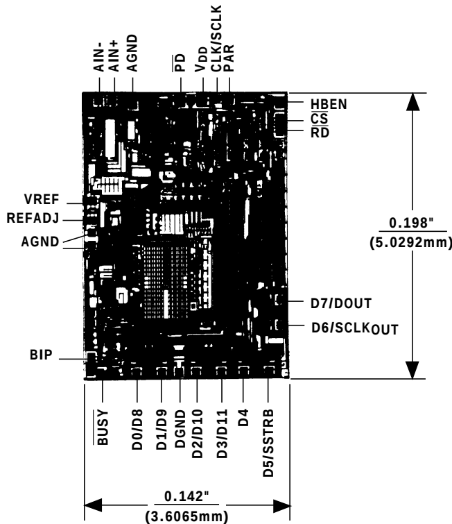
Chip Topography
