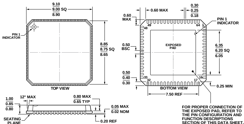
Figure 59. 64-Lead Lead Frame Chip Scale Package [LFCSP_VQ] 9 mm × 9 mm Body, Very Thin Quad (CP-64-4)
