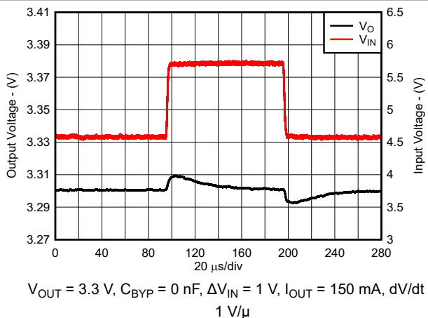
Figure 7-10. Line Transient Response for New Chip
