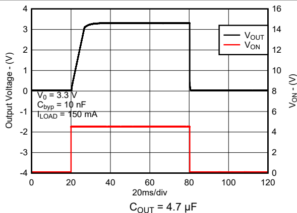
Figure 7-24. Turn-On Time for New Chip
