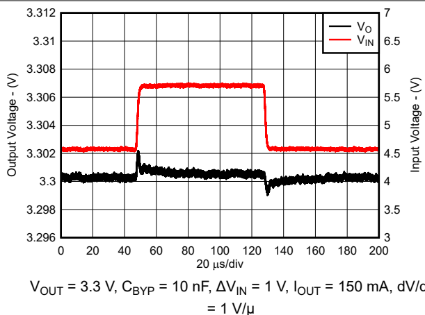
Figure 7-12. Line Transient Response for New Chip
