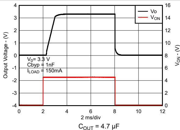
Figure 7-22. Turn-On Time for New Chip
