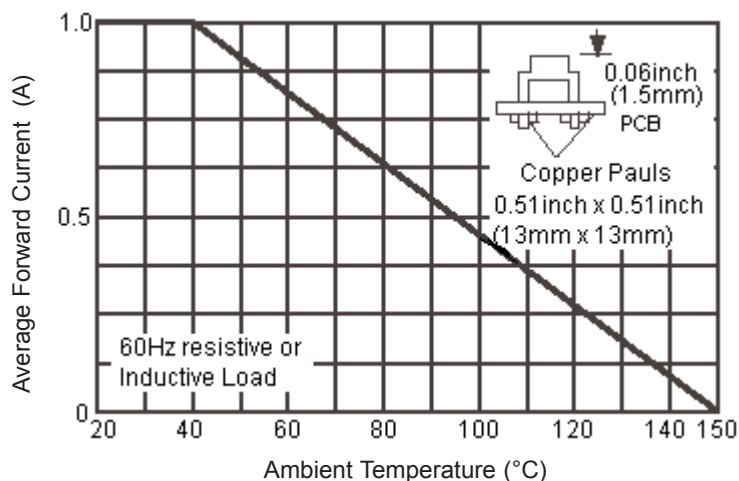
Maximum Derating Curve for Output Rectified Current
