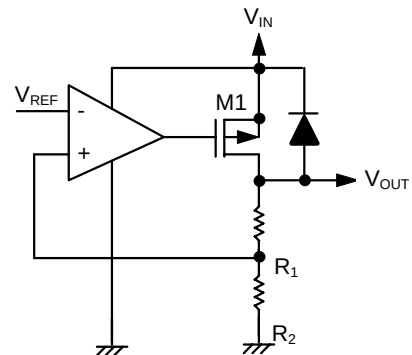
Figure 7 Voltage Regulator
