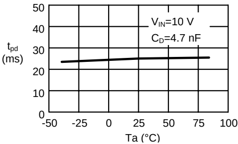
(a) Delay Time (t pd ) - Temperature (T a )
