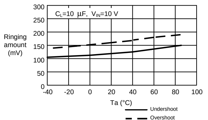
4. Temperature Dependency
