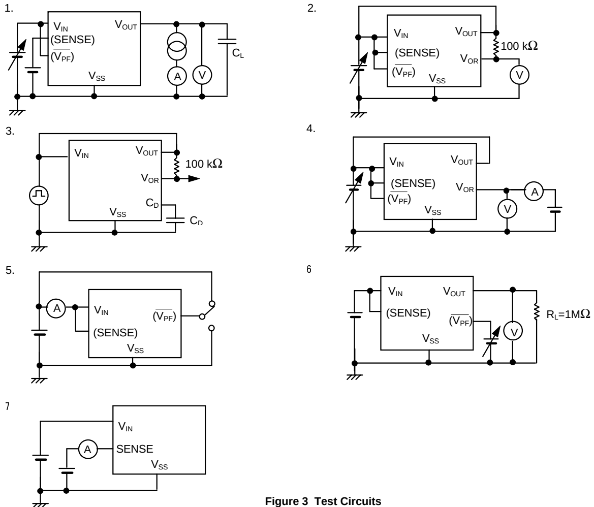
Figure 3 Test Circuits
