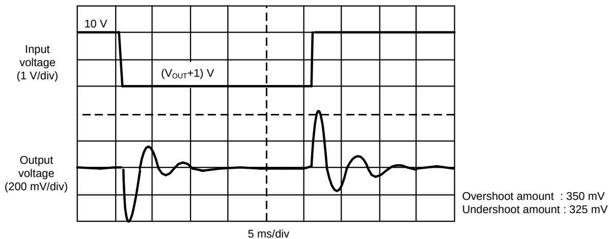
Figure 14 Type I Ringing Waveform
