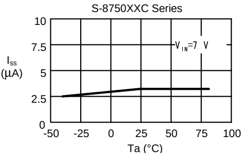
(b) Current Consumption (I ss ) - Temperature (T a )
