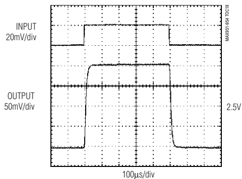
MAX952/MAX954 OP AMP SMALL-SIGNAL TRANSIENT RESPONSE
