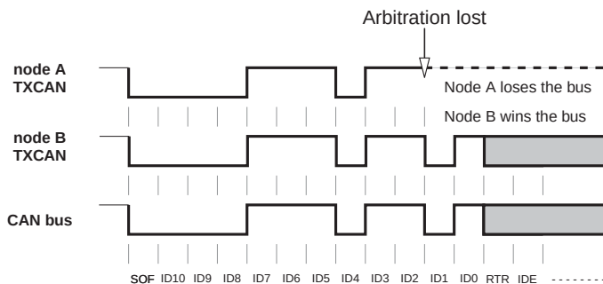
Figure 35. Bus Arbitration
