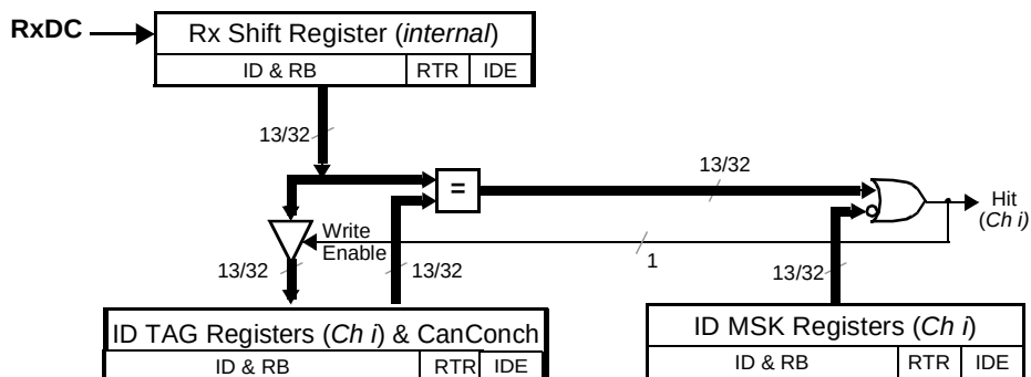
Figure 43. Acceptance Filter Block Diagram
