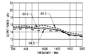
Output Power*
