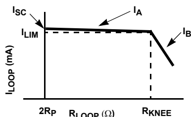
FIGURE 6. I_{\text{LOOP}} vs R_{\text{LOOP}} LOAD CHARACTERISTIC
