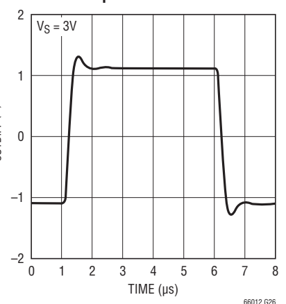
Pulse Response
