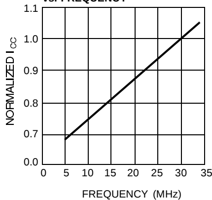
NORMALIZED I_{CC} vs. FREQUENCY
