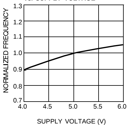
NORMALIZED FREQUENCY vs. SUPPLY VOLTAGE
