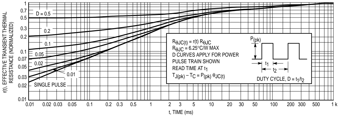
Figure 1. Thermal Response
