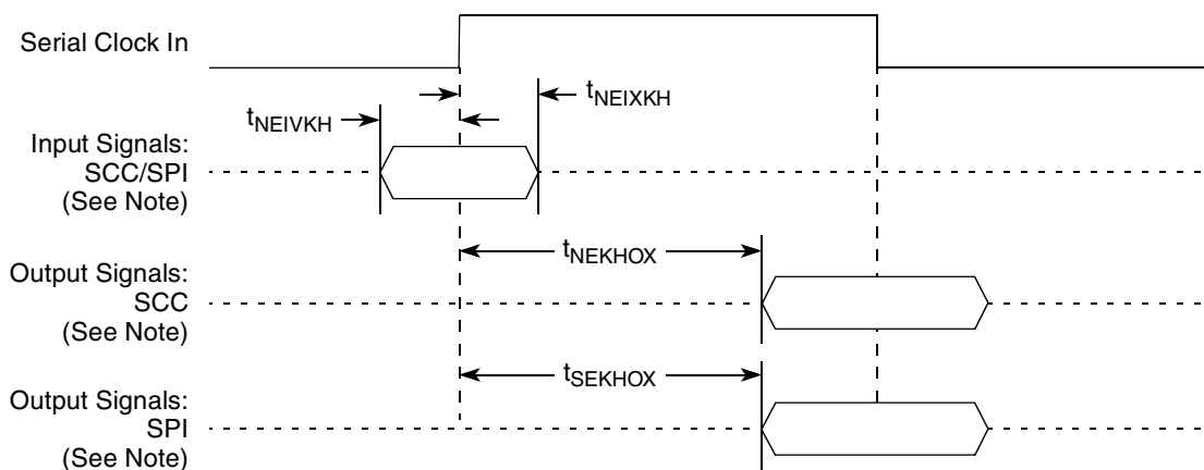
Figure 27. SCC/SPI AC Timing External Clock Diagram
