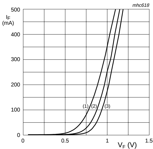
(1) T_{amb} = 150\text{ °C} (2) T_{amb} = 75\text{ °C} (3) T_{amb} = 25\text{ °C} Fig 1. Forward current as a function of forward voltage; typical values
