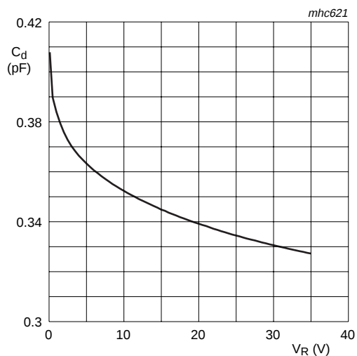
f = 1\text{ MHz} ; T_{amb} = 25\text{ °C} Fig 4. Diode capacitance as a function of reverse voltage; typical values
