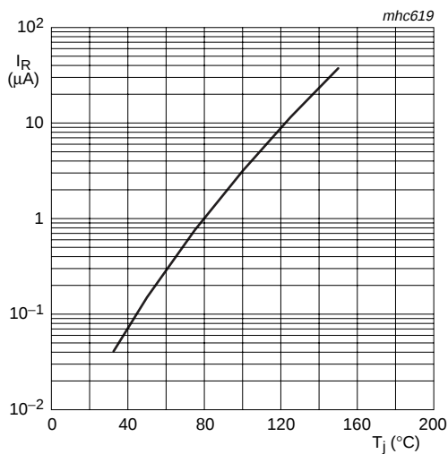
V_R = 250\text{ V} Fig 3. Reverse current as a function of junction temperature; typical values
