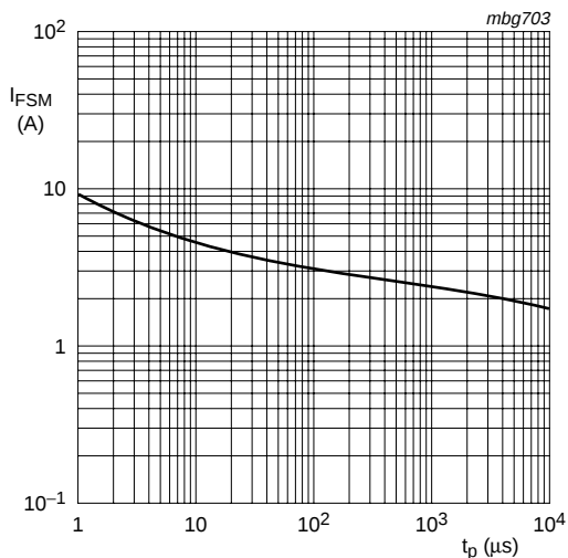
Based on square wave currents. T_j = 25\text{ °C} ; prior to surge Fig 2. Non-repetitive peak forward current as a function of pulse duration; maximum values
