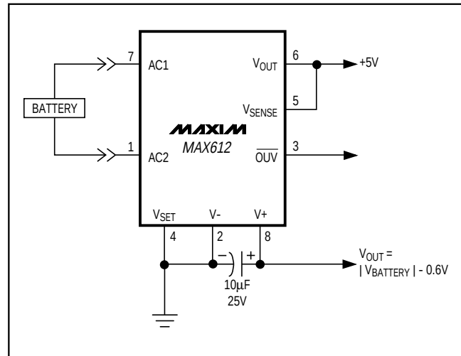
Figure 12. Polarly Insensitive Battery-Powered Supply
