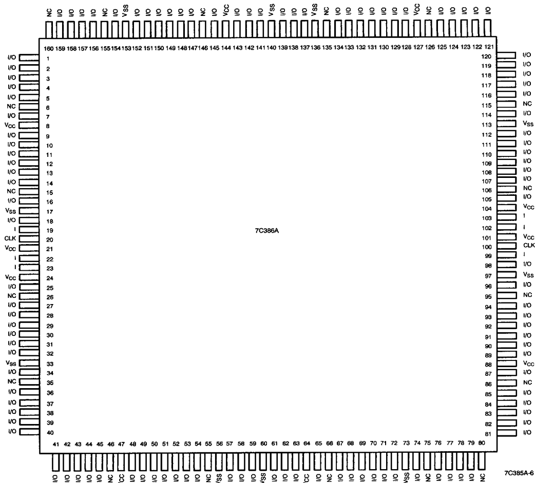
QFP Top View
