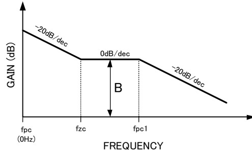
Figure 23. Feedback Transfer Function
