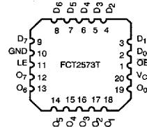
LCC Top View
