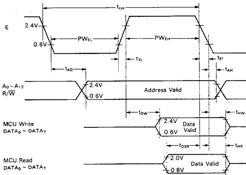
Figure 1 Bus Timing
