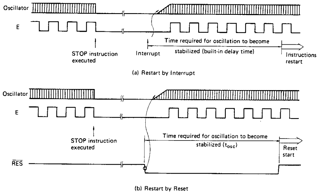
Figure 25 Timing Chart of Releasing from Stop Mode
