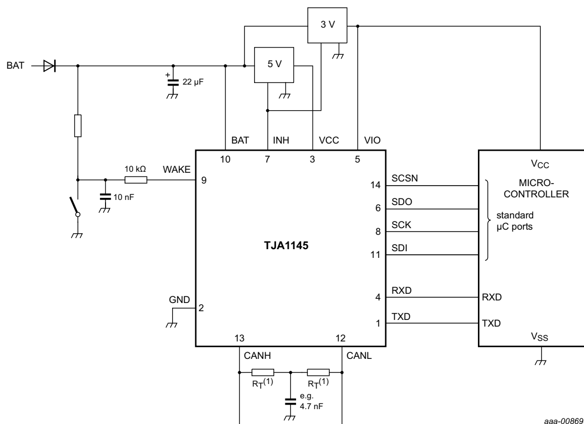
Fig 14. Typical application using the TJA1145
