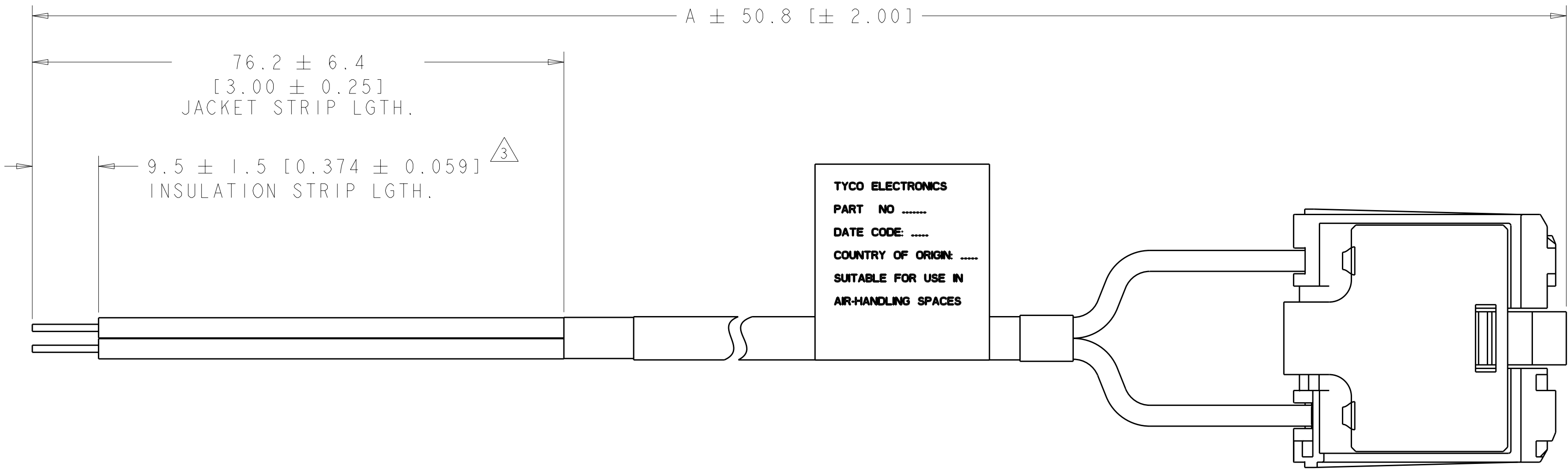
CABLE ASSEMBLY (PREPARED END) (P/N'S: 2106718-3 & -4)
