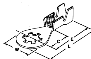
E Anti-Rotational
