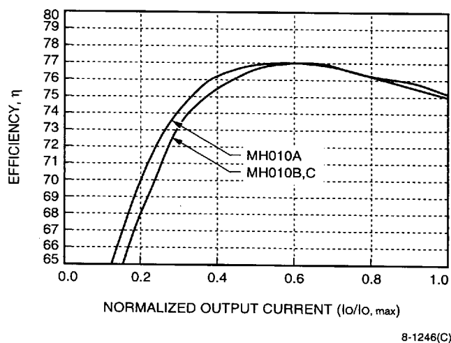
Figure 7. MH010A, B, C Typical Converter Efficiency as a Function of Output Current with V_I = 5\text{ V} and T_A = 25\text{ }^{\circ}\text{C}
