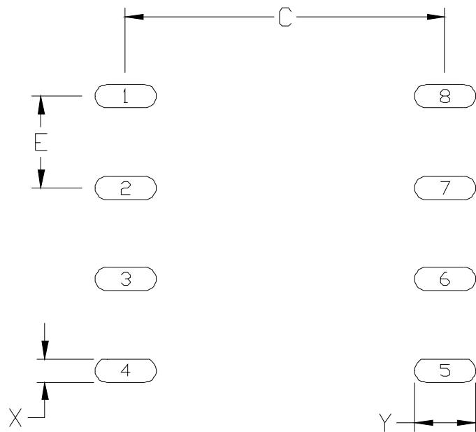
Figure 20. DIP8 Land Pattern
