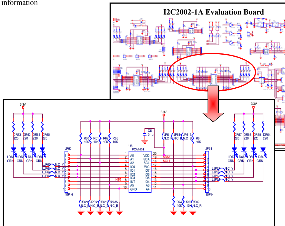
Figure 7. PCA9501 Schematic
