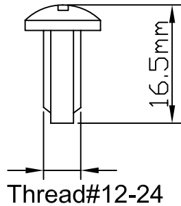
Screw
