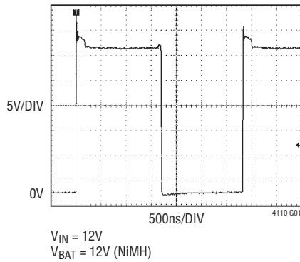
Typical CHGFET and DCHFET Waveforms
