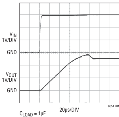
Figure 1. Turn-On Characteristics of LT6654-2.5
