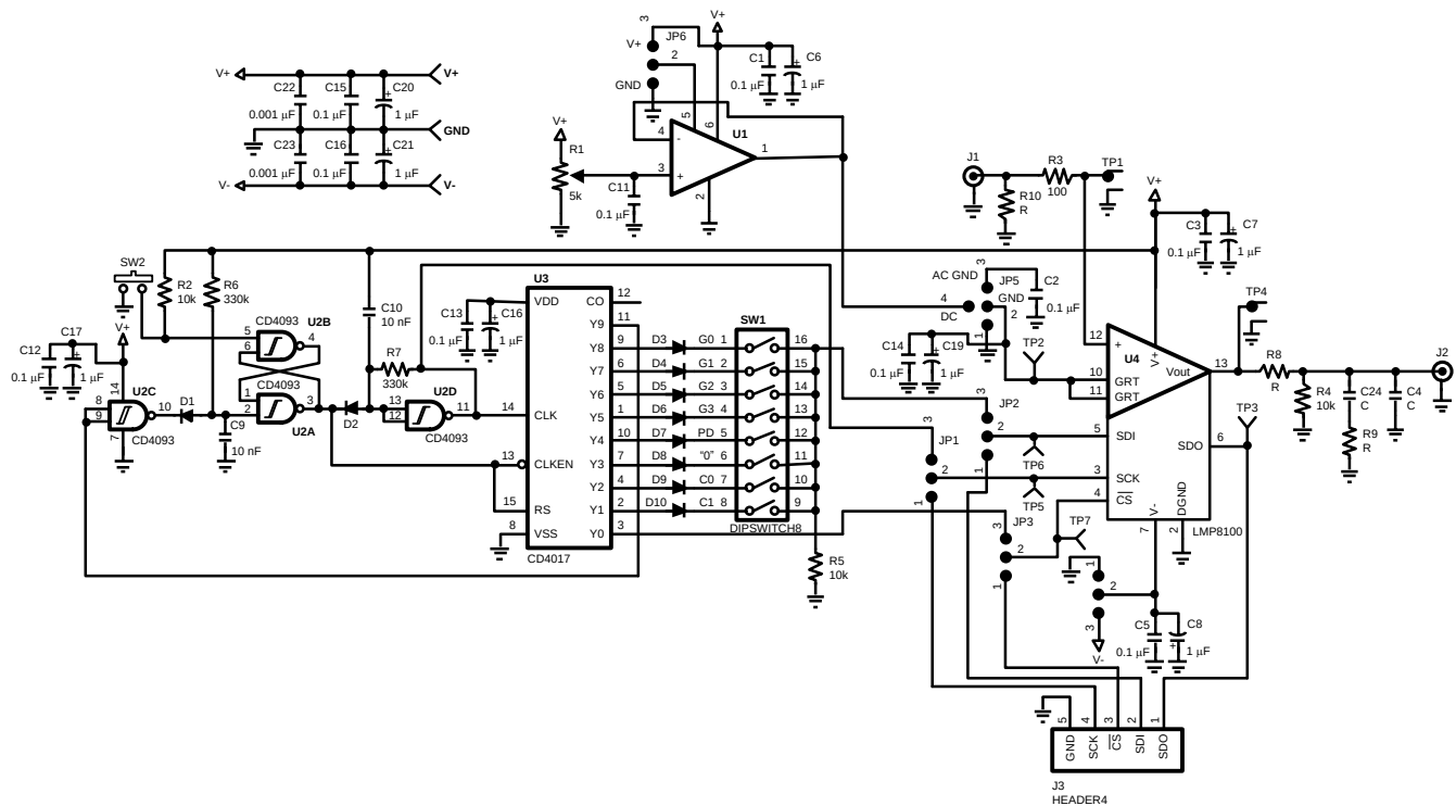
Figure 1. Schematic
