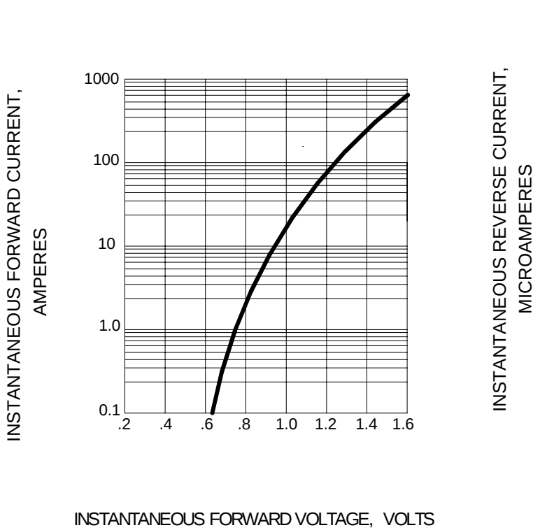
FIG.3 – TYPICAL FORWARD CHARACTERISTIC
