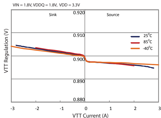
0.9V VTT Regulation Sink/Source
