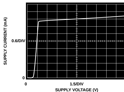
FIGURE 18. SUPPLY CURRENT vs SUPPLY VOLTAGE
