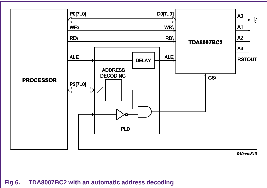
Fig 5. Typical implementation
