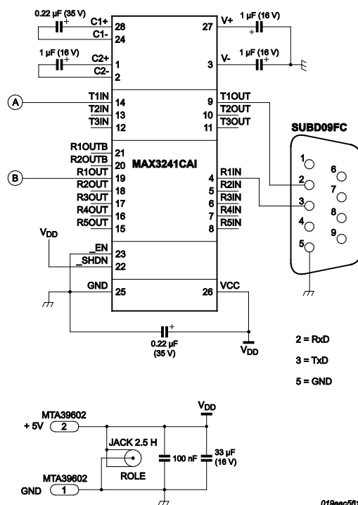
Fig 23. Reference application schematics – 3 slots, part 2
