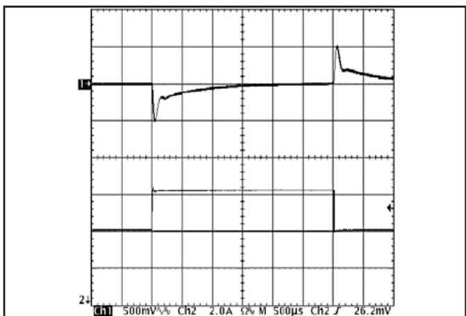
Figure 12: Output voltage response to step-change in load current (50%-75%-50% of I_{out(max)} ; dI/dt = 5A/\mu s ). Load cap: 100μF, 30 mΩ ESR tantalum capacitor and 1μF ceramic cap. Ch 1: V_{out} (500mV/div), Ch 2: I_{out} (2A/div).
