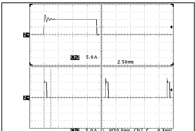
Figure 18: Load current (5A/div) as a function of time when the converter attempts to turn on into a 10 m \Omega short circuit. Top trace (2.5ms/div) is an expansion of the on-time portion of the bottom trace.
