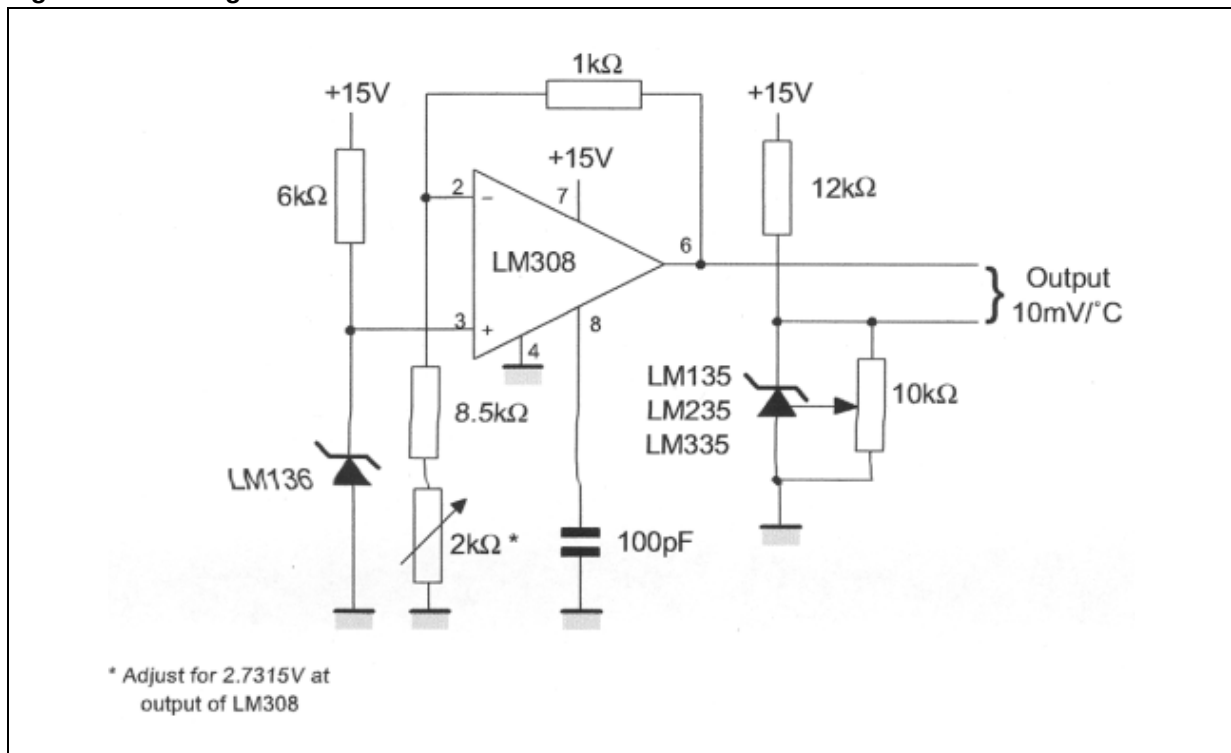
Figure 19. Centigrade thermometer
