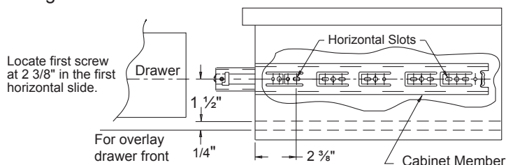
Figure 1 Conventional Mounting—Cabinet
