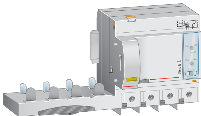
4 P - 125 A add-on module - Adjustable version
