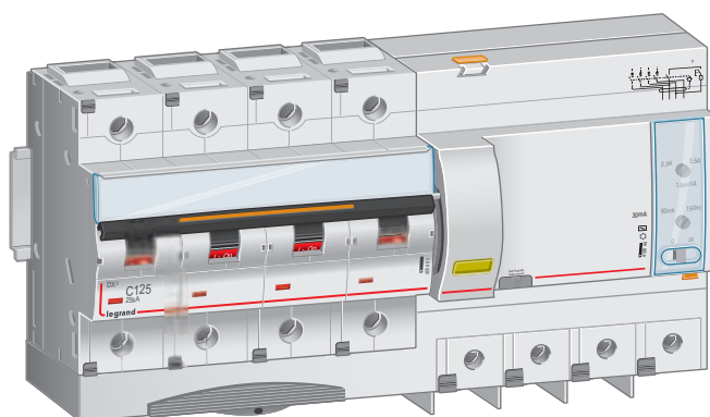
DX 3 25 kA 4-pole with add-on module
