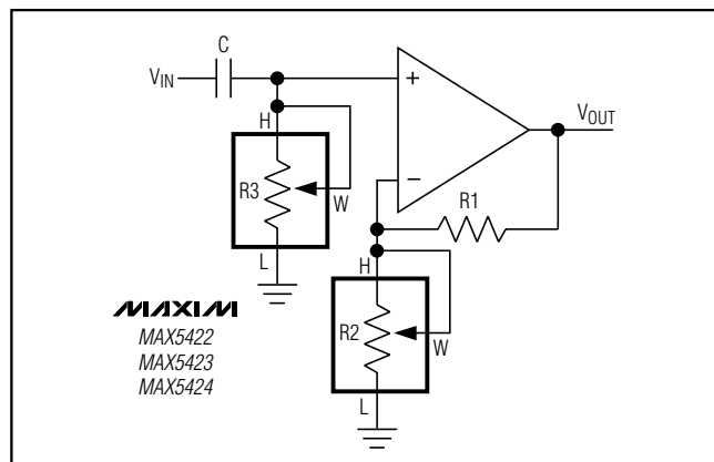
Figure 5. Programmable Filter
