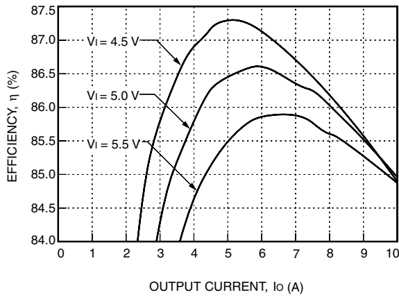
Figure 19. NH033S1R8-L Efficiency, T_A = 25^\circ\text{C}
