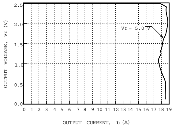
Figure 13. NH033G-L Current Limit, T_A = 25\text{ }^{\circ}\text{C}
