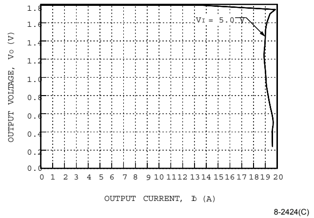
Figure 11. NH033S1R8-L Current Limit, T_A = 25^\circ\text{C}
