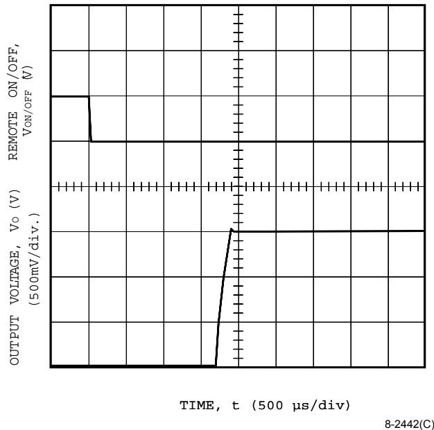
Figure 26. NH050M-L Typical Start-Up from Remote On/Off, V_i = 5\text{ V} , I_o = 15\text{ A}
