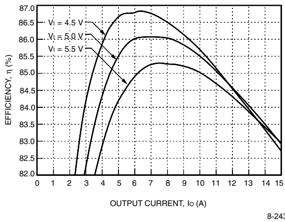
Figure 20. NH050S1R8-L Efficiency, T_A = 25^\circ\text{C}
