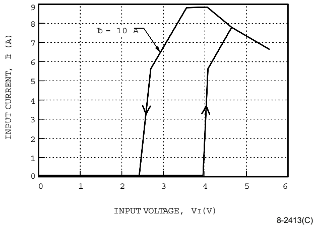
Figure 7. NH033F-L Input Characteristics, T_A = 25^\circ\text{C}
