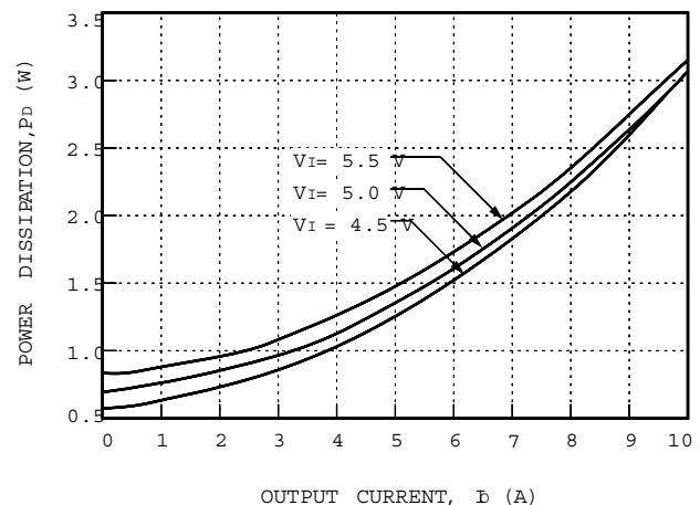
Figure 42. NH033M-L Typical Power Dissipation vs. Output Current, T_a = 25\text{ °C}
