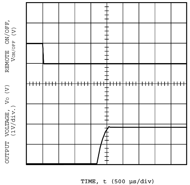
Figure 28. NH050S1R8-L Typical Start-Up from Remote On/Off, V_i = 5\text{ V} , I_o = 15\text{ A}
