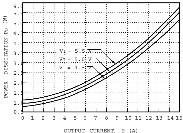
Figure 47. NH050G-L Typical Power Dissipation vs. Output Current, T_A = 25^\circ\text{C}
