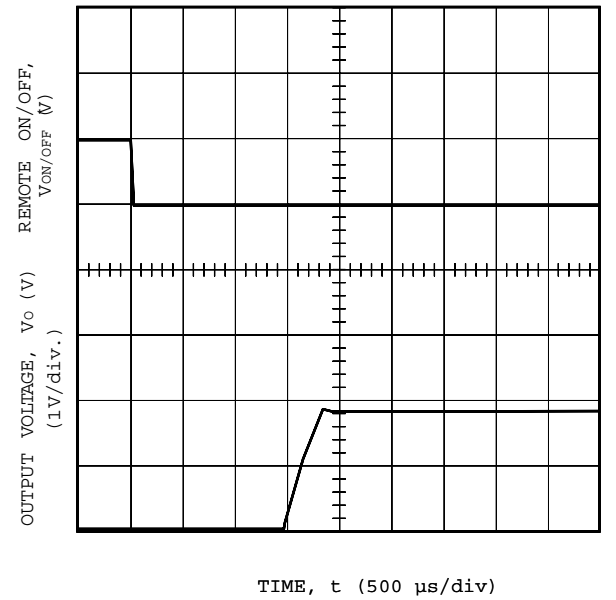
Figure 27. NH033S1R8-L Typical Start-Up from Remote On/Off, V_i = 5\text{ V} , I_o = 10\text{ A}
