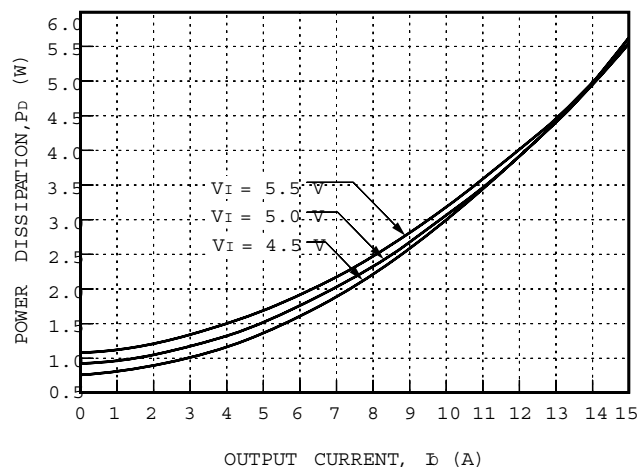
Figure 45. NH050S1R8-L Typical Power Dissipation vs. Output Current, T_A = 25\text{ °C}
