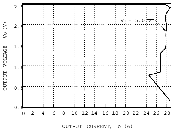
Figure 14. NH050G-L Current Limit, T_A = 25\text{ }^{\circ}\text{C}
