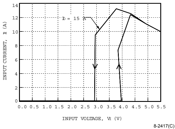
Figure 8. NH050F-L Input Characteristics, T_A = 25^\circ\text{C}
