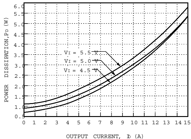
Figure 49. NH050F-L Typical Power Dissipation vs. Output Current, T_A = 25^\circ\text{C}
