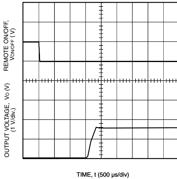
Figure 25. NH033M-L Typical Start-Up from Remote On/Off, V_i = 5\text{ V} , I_o = 10\text{ A}
