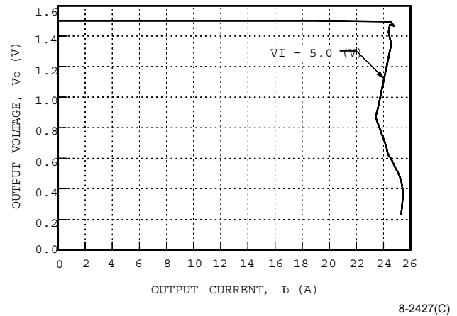
Figure 10. NH050M-L Current Limit, T_A = 25^\circ\text{C}
