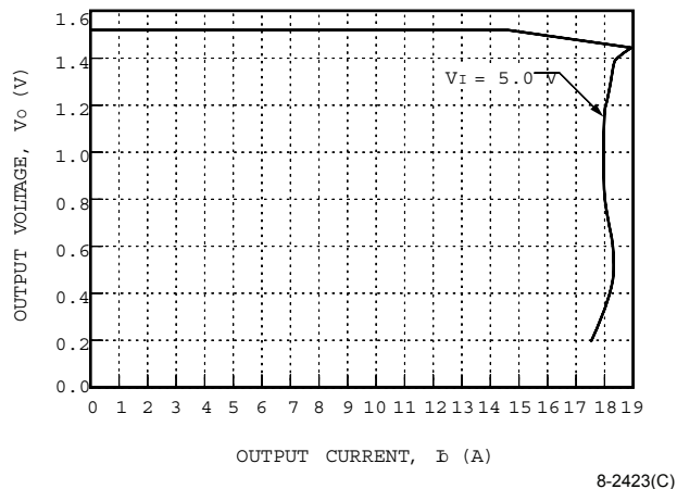
Figure 9. NH033M-L Current Limit, T_A = 25^\circ\text{C}
