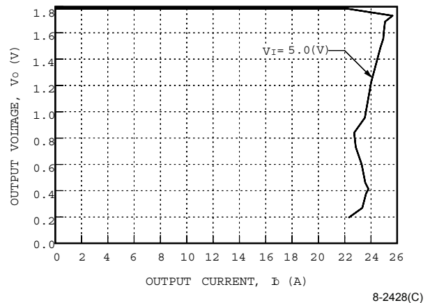
Figure 12. NH050S1R8-L Current Limit, T_A = 25^\circ\text{C}
