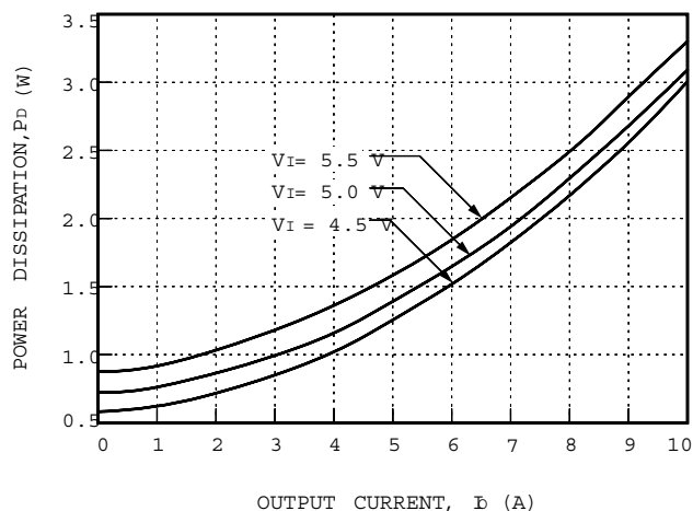
Figure 48. NH033F-L Typical Power Dissipation vs. Output Current, T_A = 25^\circ\text{C}
