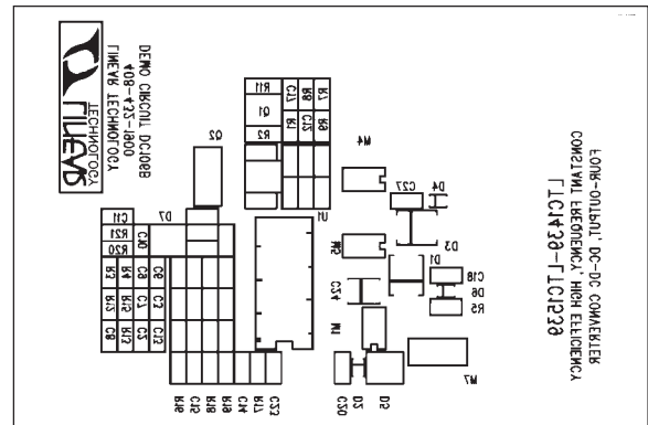
Silkscreen Bottom
