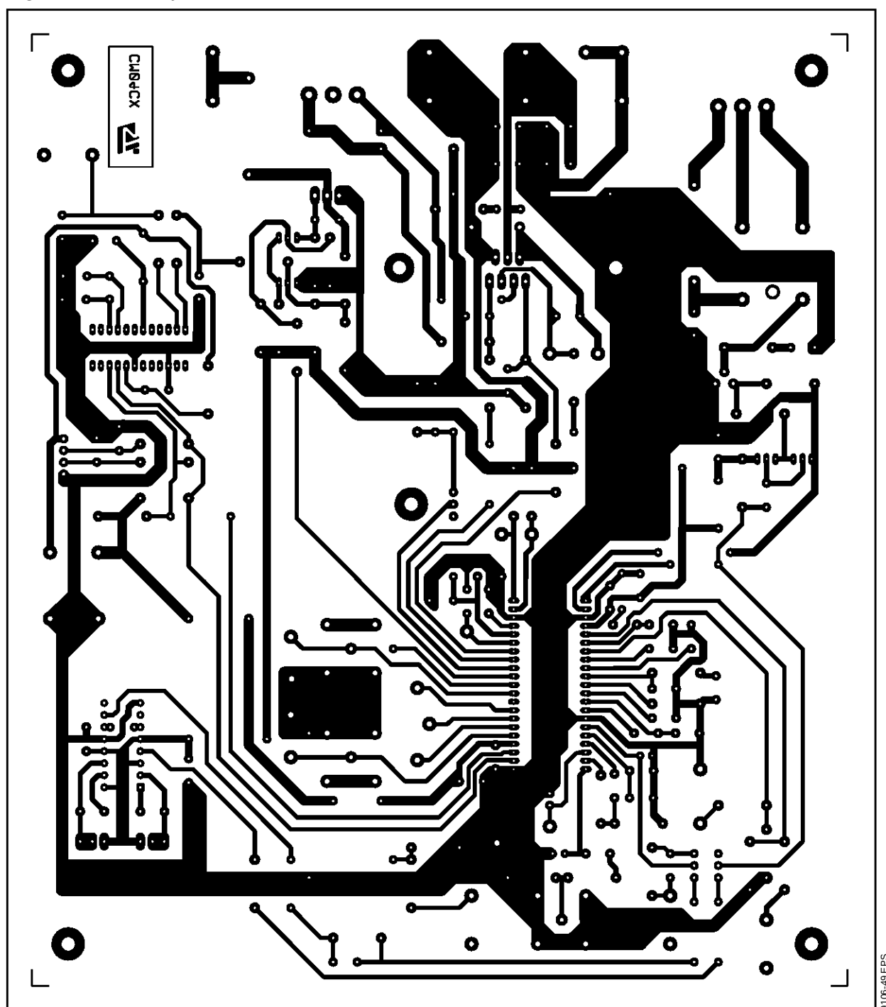
Figure 24 : PCB Layout
