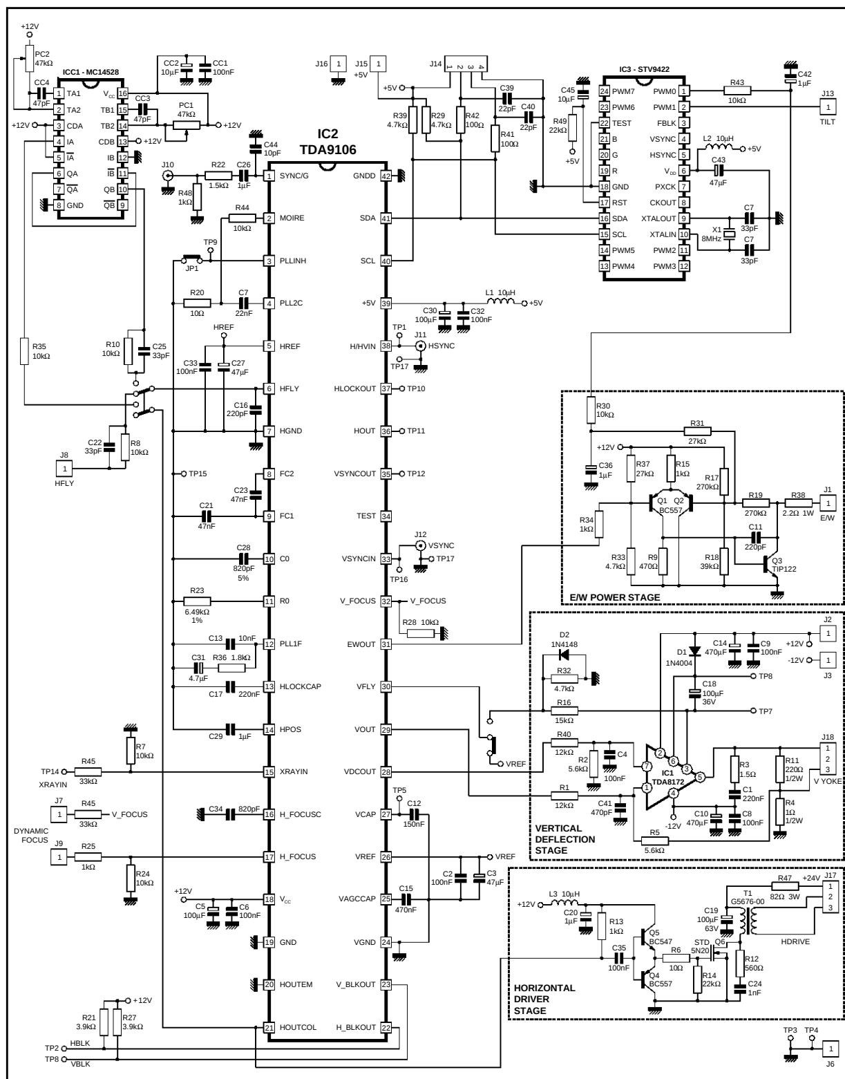
Figure 23 : Demonstration Board
