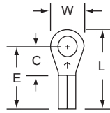
11-6S Stud Size 6 Wire Range 22-18
