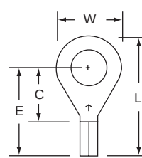
11-14S Stud Size 1/4 Wire Range 22-18
