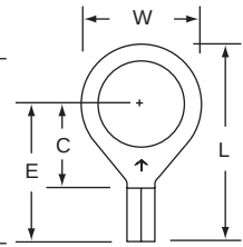
11-38 Stud Size 3/8 Wire Range 22-18
