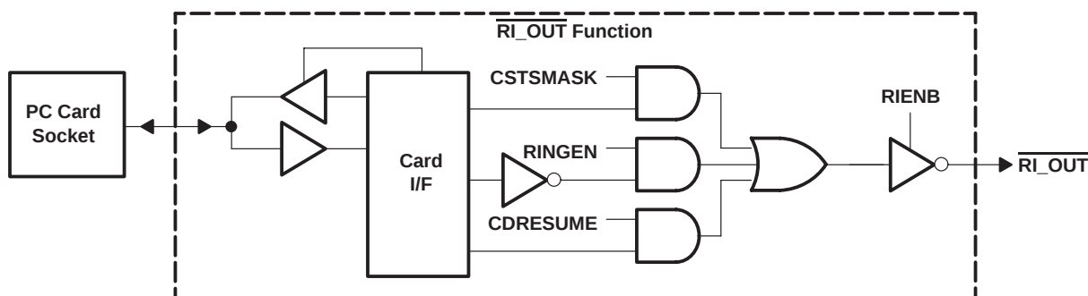
Figure 18. \overline{\text{RI\_OUT}} Functional Diagram
