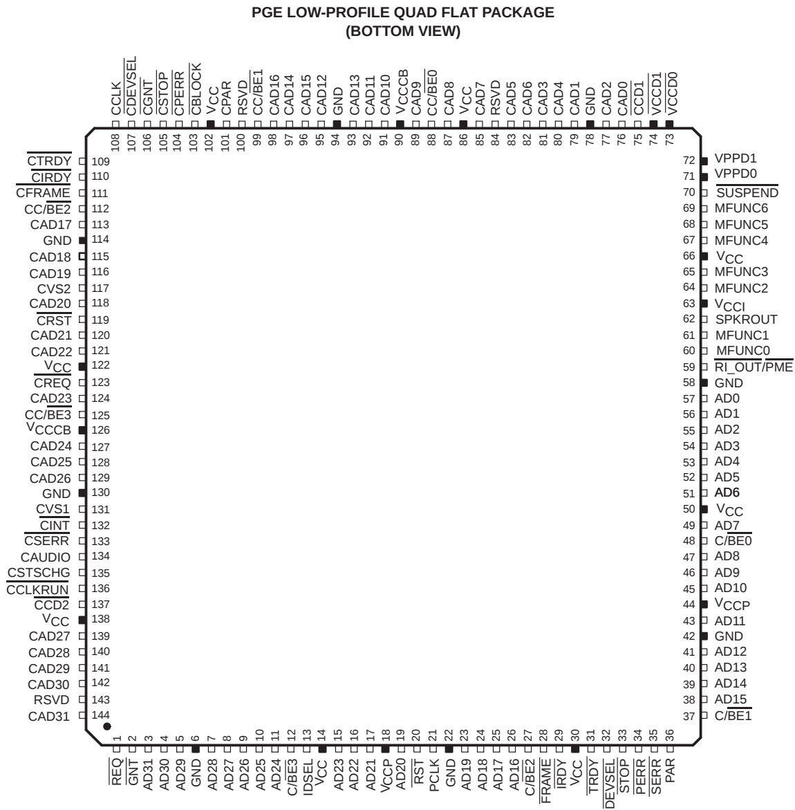
PCI-to-CardBus Pin Diagram
