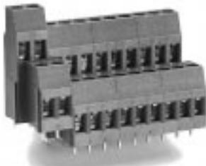
AKZ750 Front Wire Entry
