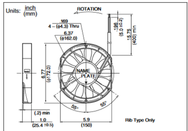
5910PL product drawing
