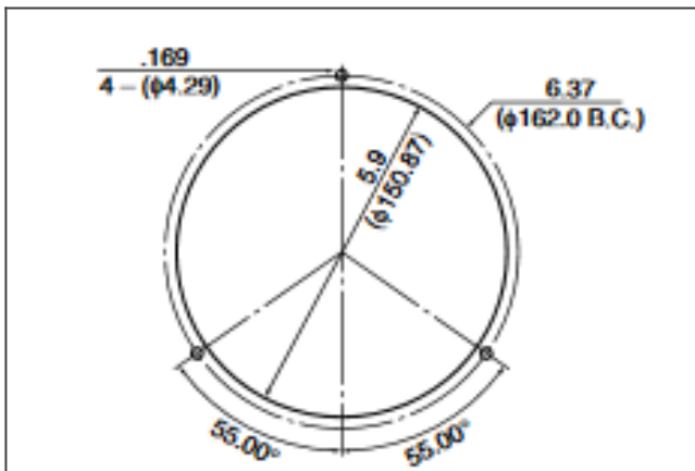
5910PL panel cut out
