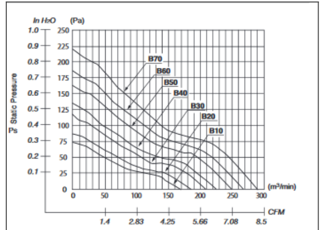
5910PL characteristic curve
