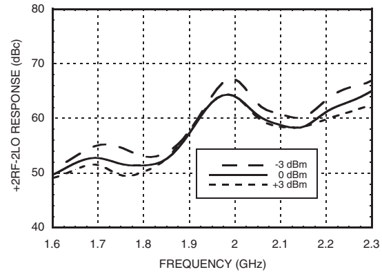
+2RF -2LO Response vs. LO Drive [3]
