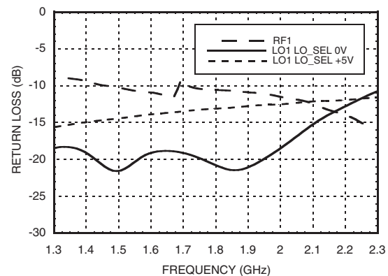
Single Channel: Return Loss
