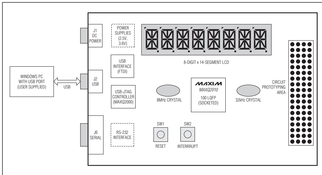
Figure 3. MAXQ2010 EV Kit Functional Layout
