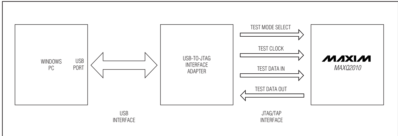
Figure 2. MAXQ2010 USB-to-JTAG Interface
