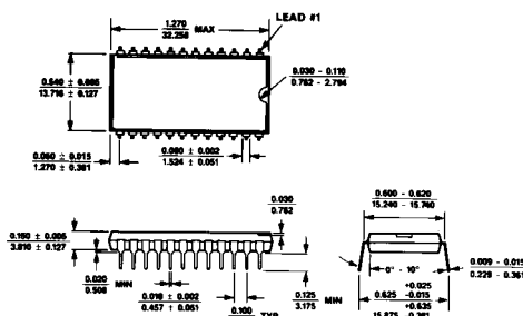
24 Lead Plastic DIP (PG)
