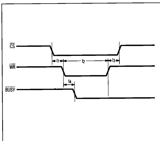
Figure 1. Start Cycle Timing
