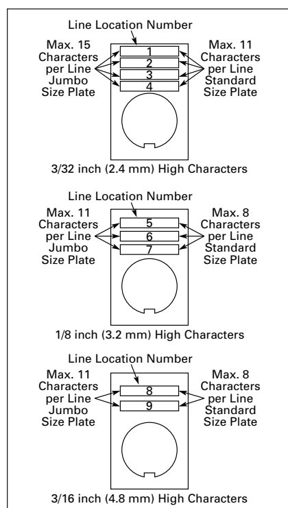
Figure 47-21. Aluminum and Plastic Legend Plates
