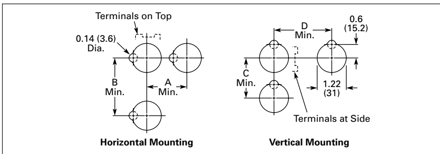
Figure 47-117. Mounting Options in Inches (mm)
