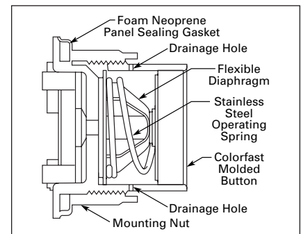
Figure 47-91. Diaphragm Seal
