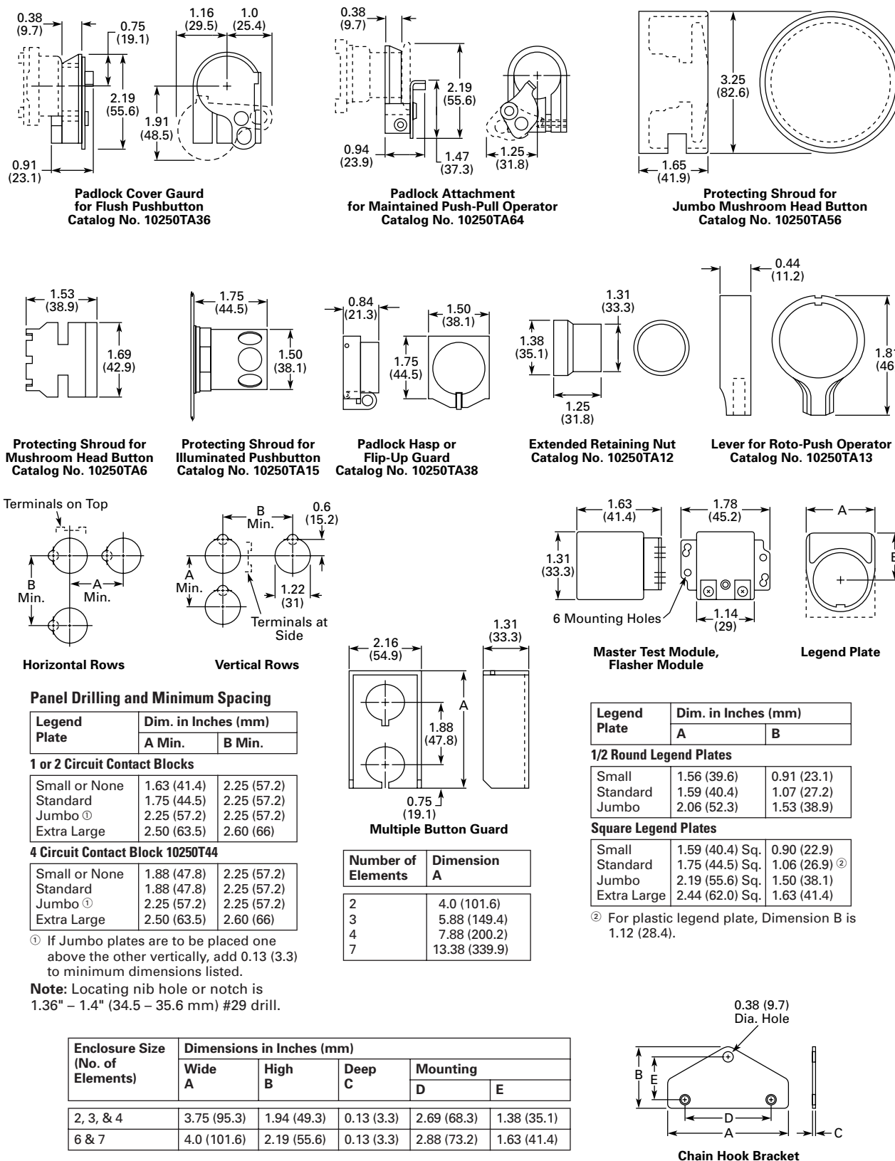
Figure 47-121. Approximate Dimensions in Inches (mm)
