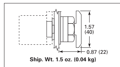
Figure 47-46. E22/EM22 Series 40 mm Dia. Push-Pull Button
