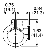
Padlock Attachment for Flush Pushbutton Catalog No. 10250TA2
