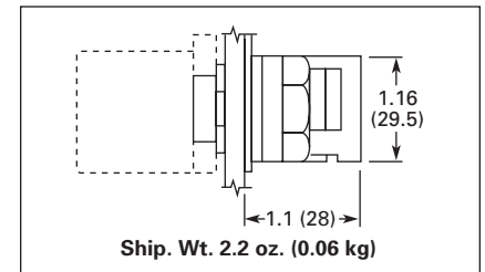
Figure 47-36. E22/EM22 Series 25 mm Dia. Extended Lens with Shroud
