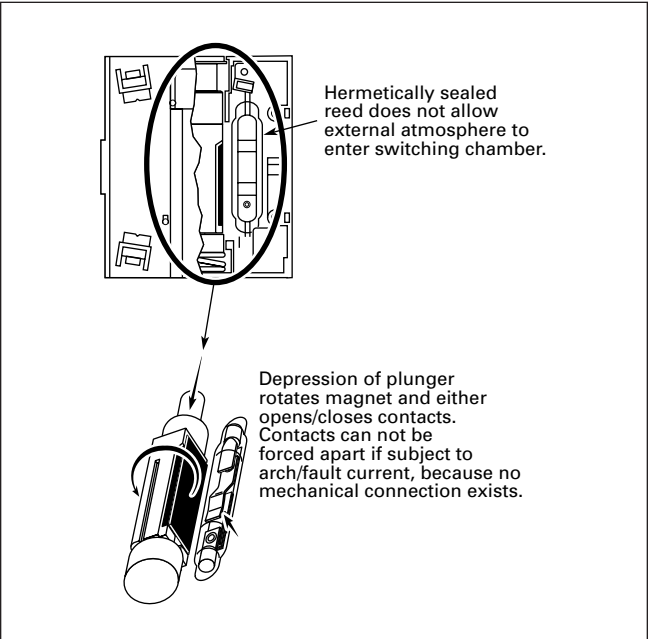
Figure 47-156. Hermetically Sealed Reed Contact Block
