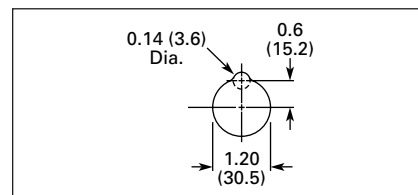
Figure 47-118. Drilling Dimensions in Inches (mm)
