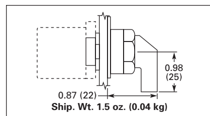
Figure 47-58. E22 Series 2-Position — 45° Throw — Lever
