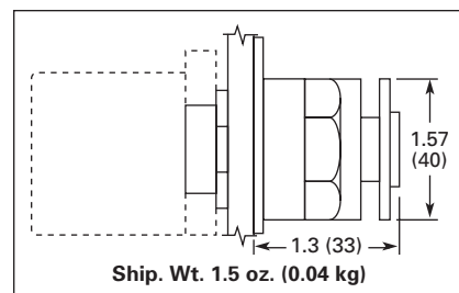
Figure 47-56. E22/EM22 Series 3-Position 40 mm Dia. Lens (Spring Return to Center)
