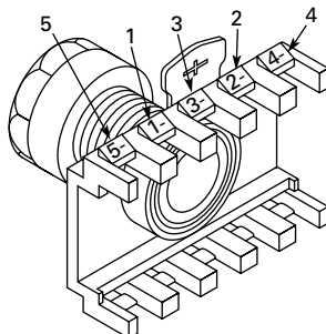
5- 1- 3- 2- 4- Contact Block Mounting Position Numbers Molded in 5-Way Mounting Adapter, See Accessories for 5-Way Adapter — Page 47-72
