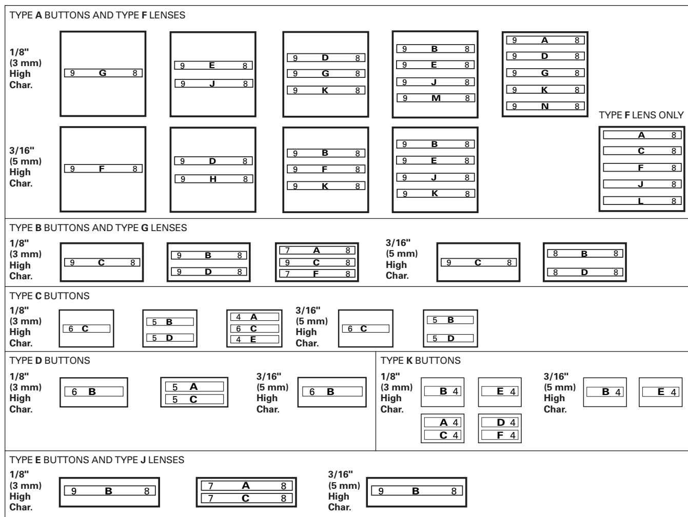
Figure 47-85. Legend Locations
