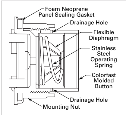
Figure 47-123. Diaphragm Seal
