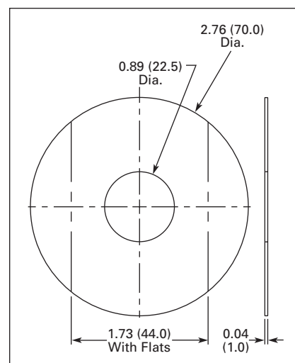
Figure 47-78. Joystick Nameplate Dimensions — Approximate Dimensions in Inches (mm)
