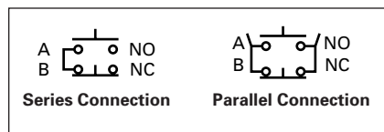
Figure 47-110. Series and Parallel Connection
