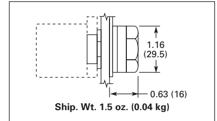
Figure 47-34. E22/EM22 Series 25 mm Dia. Flush Lens
