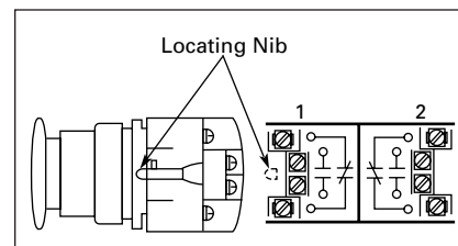
Figure 47-145. Locating Nibs
