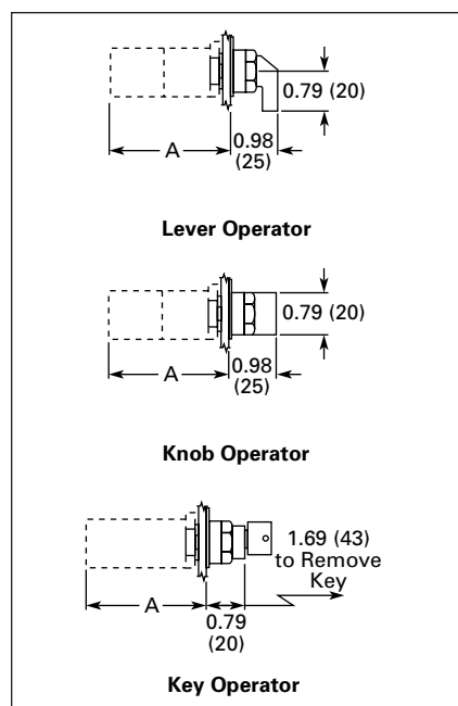
Figure 47-26. Approximate Dimensions in Inches (mm)
