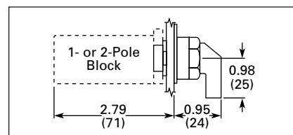
Figure 47-73. Rotary Cam Selector Switch For each additional (1- or 2-pole) block add 0.47" (12 mm).
