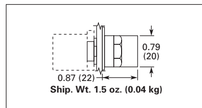
Figure 47-72. EM22 Series — 60° Throw — Knob
