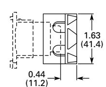
Padlock Attachment for Knob Selector Switch Catalog No. 10250TA11
