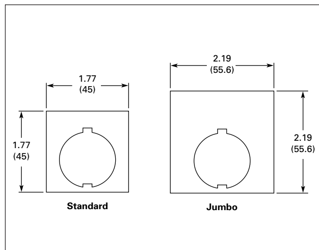
Figure 47-143. Legend Plates — Approximate Dimensions in Inches (mm)
