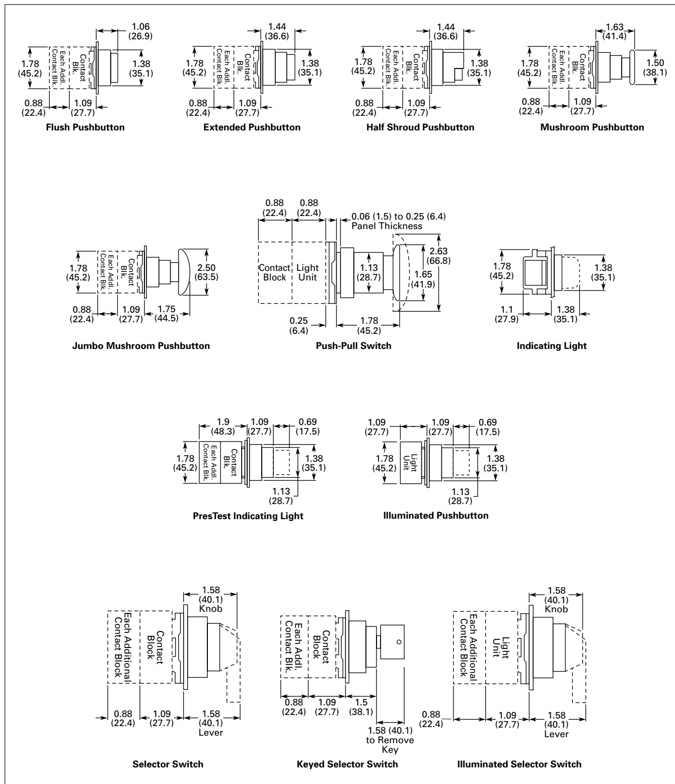
Figure 47-134. Approximate Dimensions in Inches (mm)
