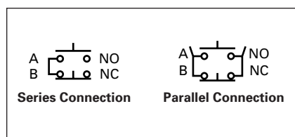
Figure 47-106. Series and Parallel Connections
