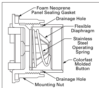
Figure 47-144. Diaphragm Seal
