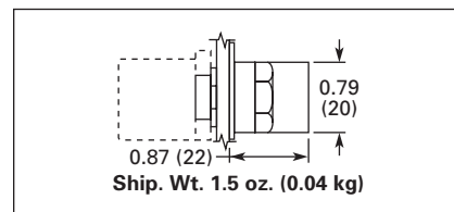
Figure 47-60. E22 Series 2-Position — 45° Throw — Knob
