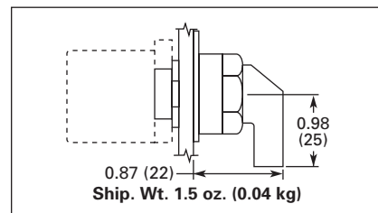
Figure 47-59. E22 Series 3-Position — 45° Throw — Lever
