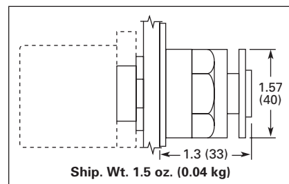
Figure 47-57. E22/EM22 Series 3-Position 40 mm Dia. Push-Pull Pushbutton (Spring Return to Center from Pulled Position)
