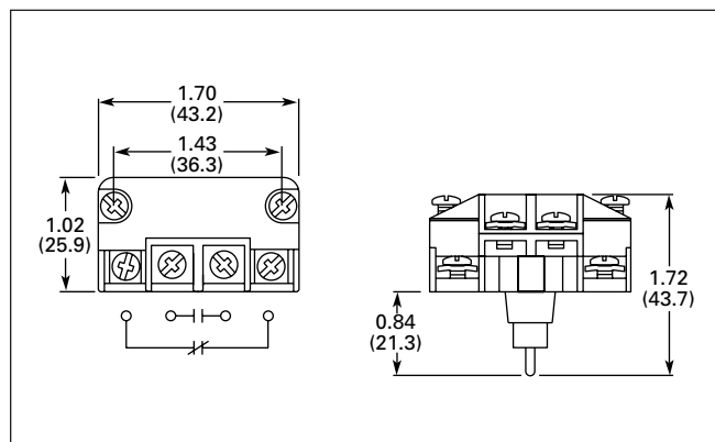
Figure 47-150. Contact Block
