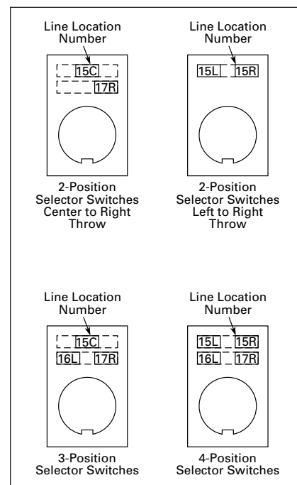
Figure 47-25. Selector Switch Legend Plates
