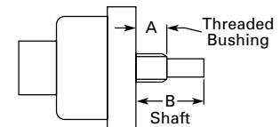
Shaft Dimensions of Potentiometer That C-H Operator Will Accept
