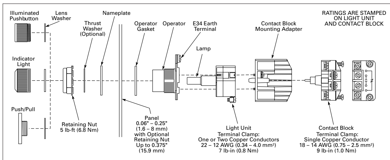
Figure 47-154. Operator Assembly
