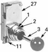
4-Position Joystick Operator (w/o Latch)
