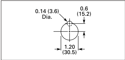
Figure 47-133. Drilling Dimensions in Inches (mm)
