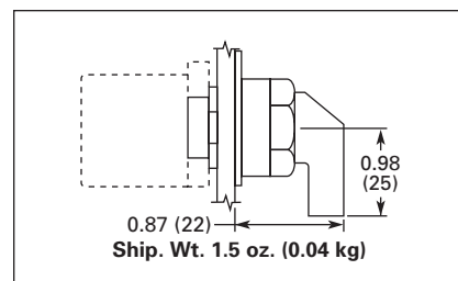
Figure 47-71. EM22 Series — 60° Throw — Lever
