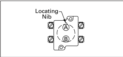
Figure 47-103. Mounting Location
