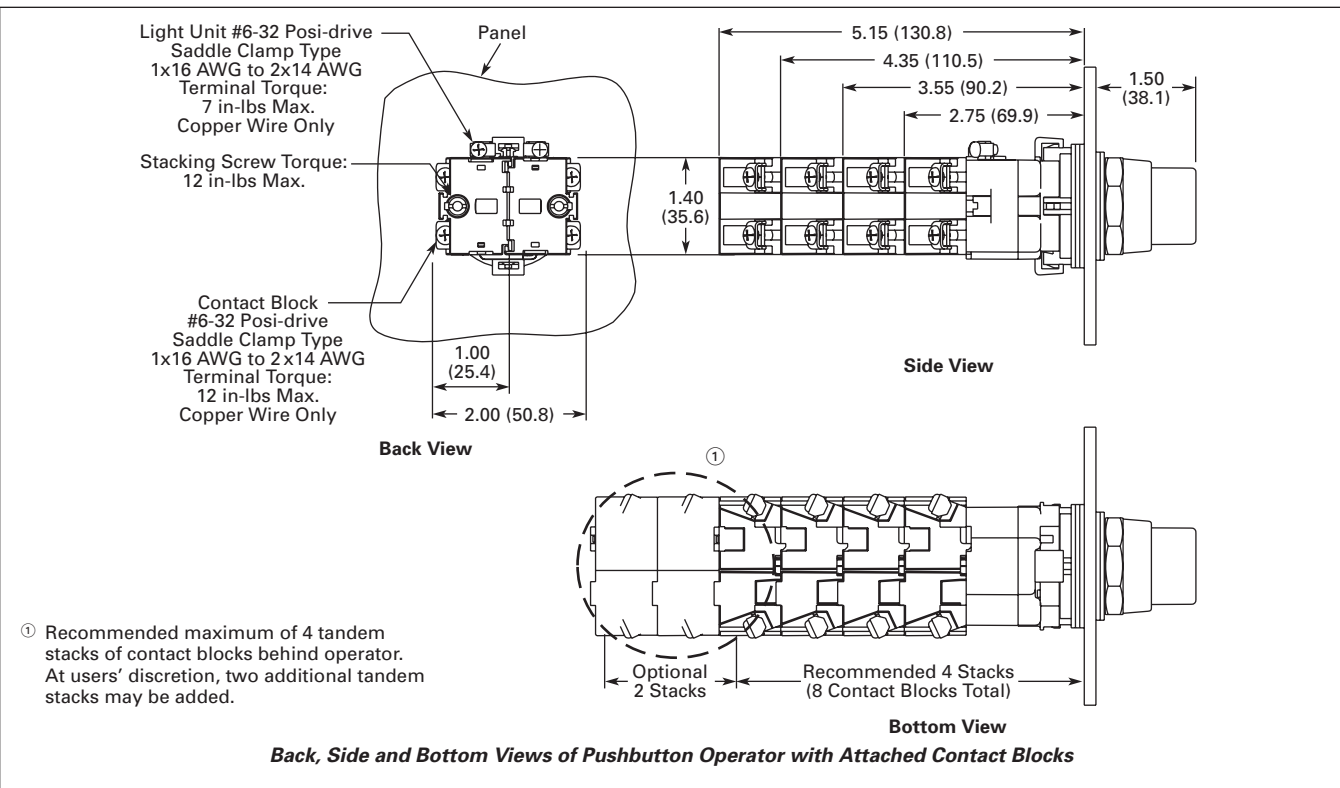
Figure 47-137. Illuminated Pushbuttons — Approximate Dimensions in Inches (mm)
