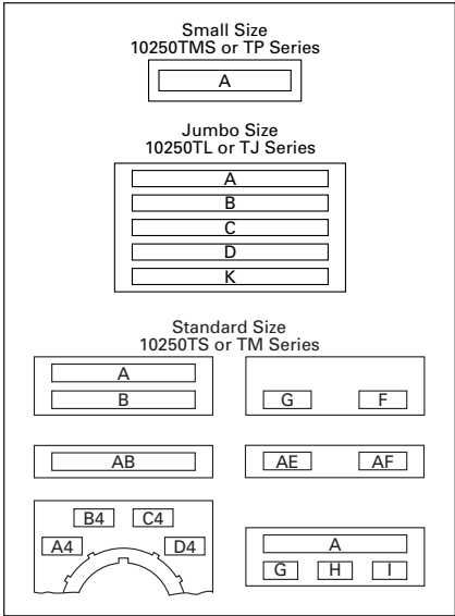
Figure 47-113. Legend Positions
