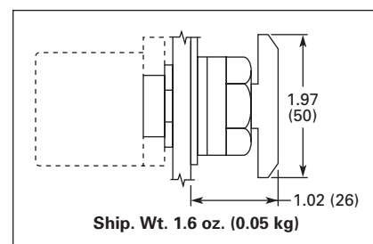
Figure 47-47. E22/EM22 Series 50 mm Dia. Push-Pull Button
