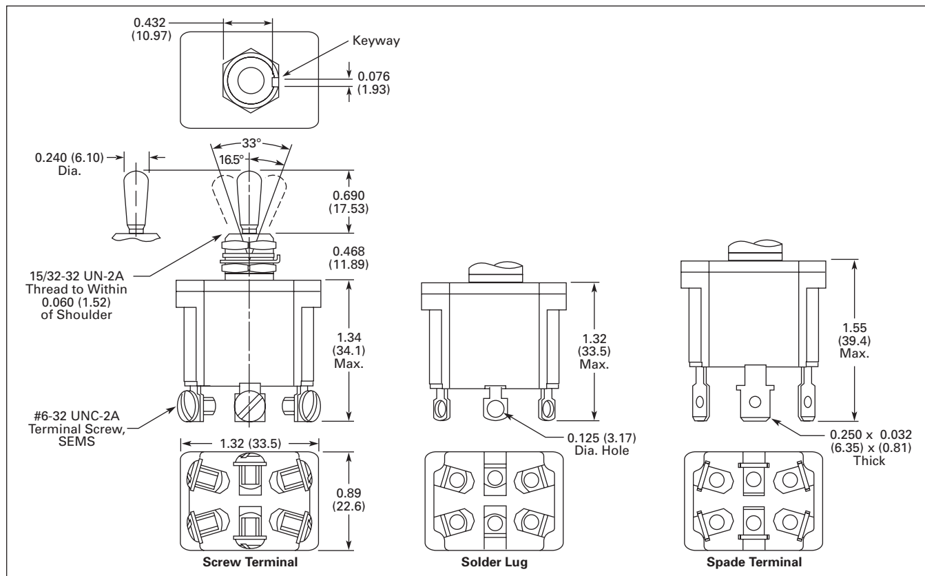
Figure 47-7. Two-Pole Econoswitch E10E Series Toggle Switches — Approximate Dimensions in Inches (mm)
