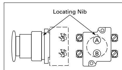
Figure 47-124. Contact Circuit Locations
