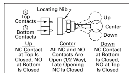
Figure 47-97. A and B Mounting Location
