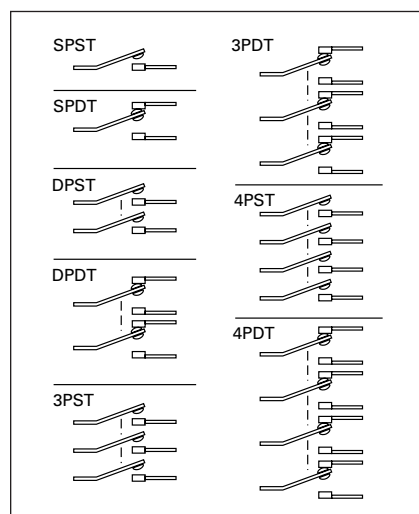
Figure 47-1. Circuit Arrangements
