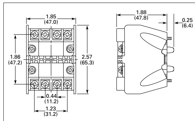
Figure 47-151. Mounting Adapter
